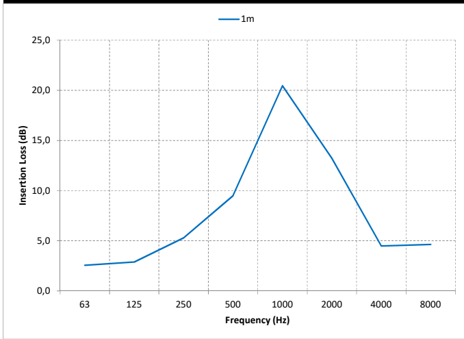
SEMI RIGID SILENCER 90/120 mic. 50mm Ins (Ø315mm)
