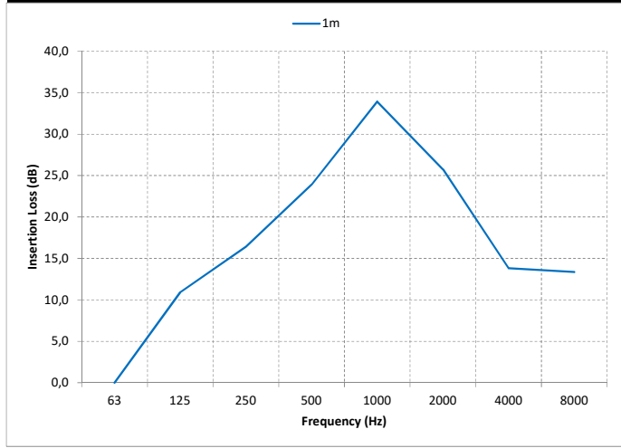
SEMI RIGID SILENCER 90/120 mic. 50mm Ins (Ø100mm)
