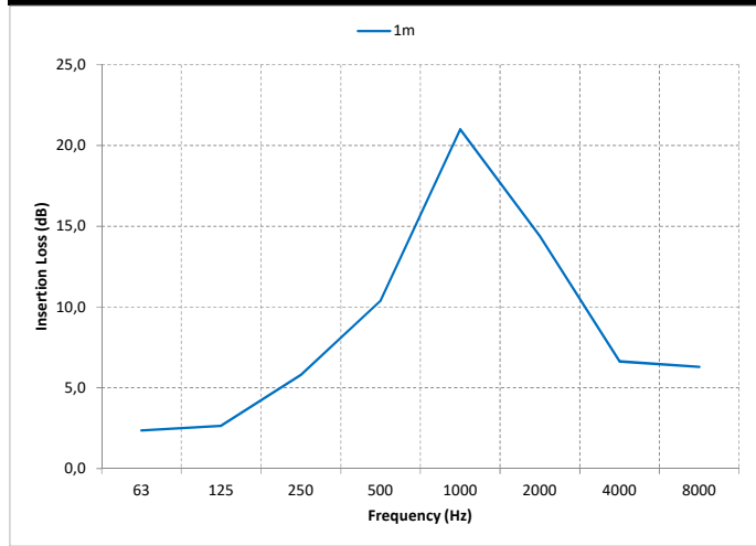
SEMI RIGID SILENCER 90/120 mic. 50mm Ins (Ø356mm)
