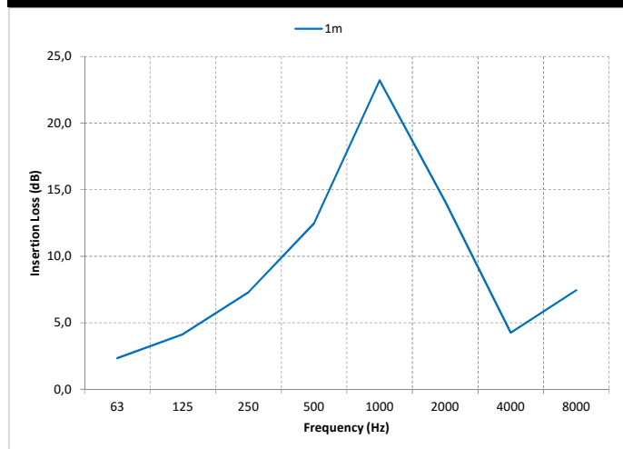
SEMI RIGID SILENCER 90/120 mic. 50mm Ins (Ø250mm)
