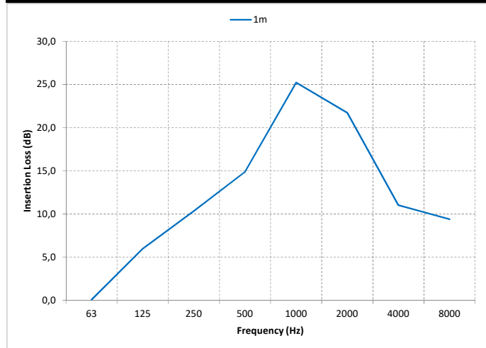
SEMI RIGID SILENCER 90/120 mic. 50mm Ins (Ø160mm)
