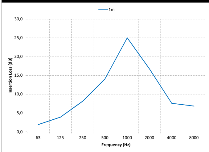
SEMI RIGID SILENCER 90/120 mic. 50mm Ins (Ø200mm)
