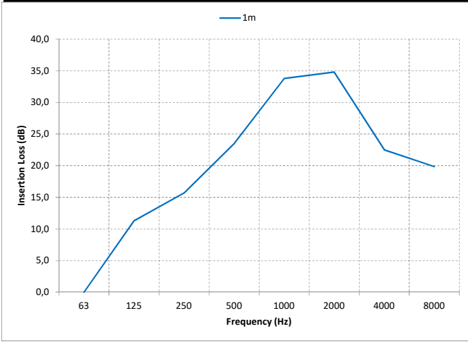
SEMI RIGID SILENCER 90/120 mic. 50mm Ins (Ø80mm)
