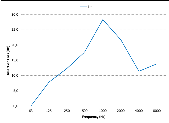
SEMI RIGID SILENCER 90/120 mic. 50mm Ins (Ø125mm)
