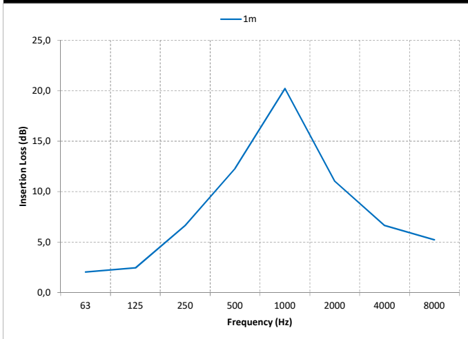
SEMI RIGID SILENCER 90/120 mic. 50mm Ins (Ø400mm)
